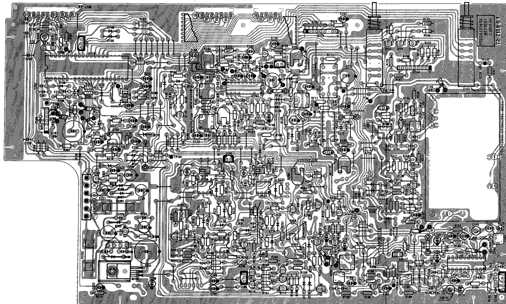
TUNER PCB
