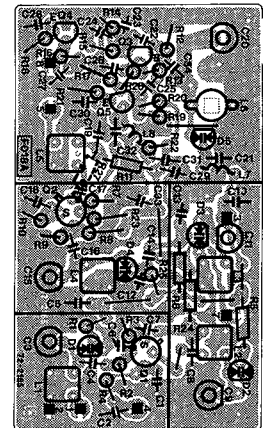
FRONTEND PCB
