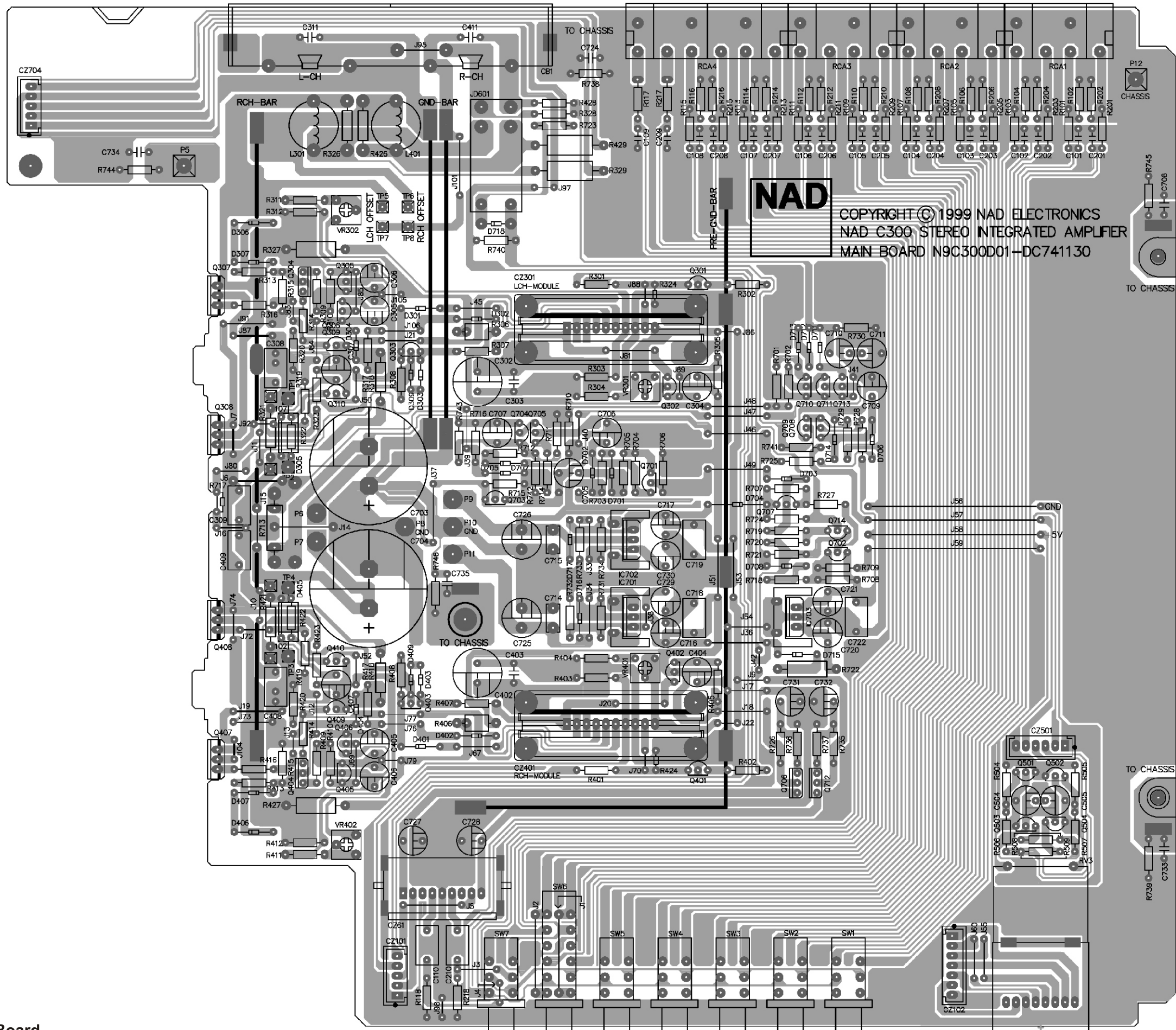
Main Board
