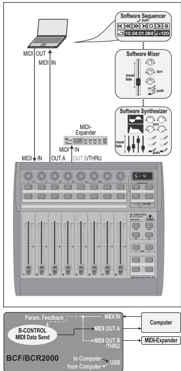
Fig. 4.9: Routing and use in stand-alone mode 4
